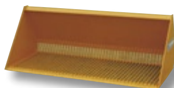
Kartoffelschaufel, offene Form Breite: 1,60m - 2,50m Inhalt: 0,61m 3 - 1,50m 3
